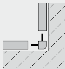
Accessory piece as external corner
